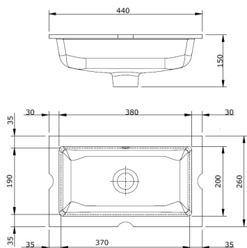
MINI AGRES 44 X 26 UNDER COUNTER CERAMIC WASH BASIN
