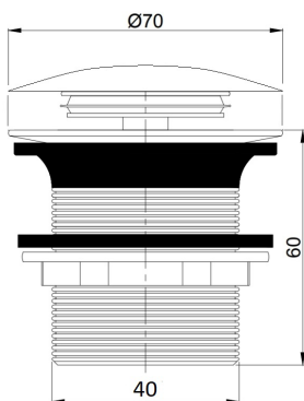
TITANCAST 40MM BATH WASTE
