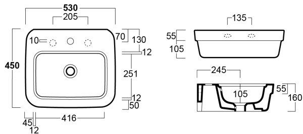
BALFOUR 53 WALL HUNG BASIN
