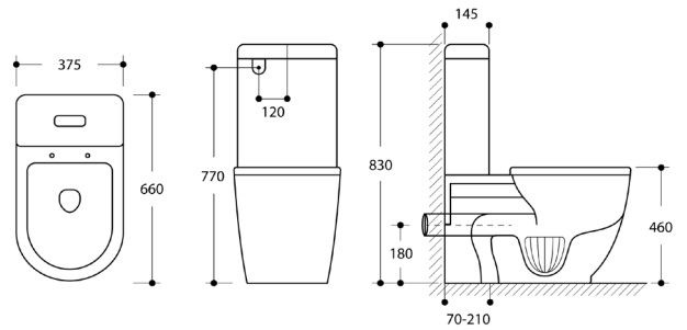
NARVA RIMLESS CLOSE COUPLED BACK TO WALL TOILET SUITE
