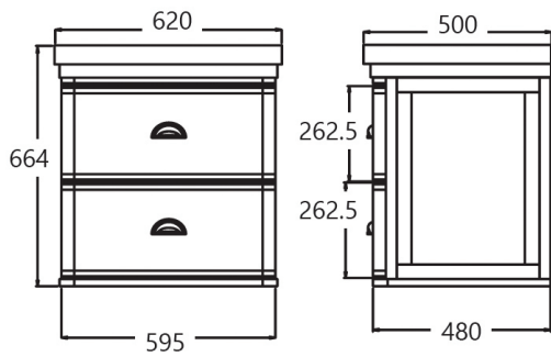
STAFFORD 62 X 50 WALL MOUNTED BASIN & VANITY
