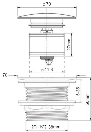
SAFETY PULL OUT BATH WASTE WITH SHORT TAIL
