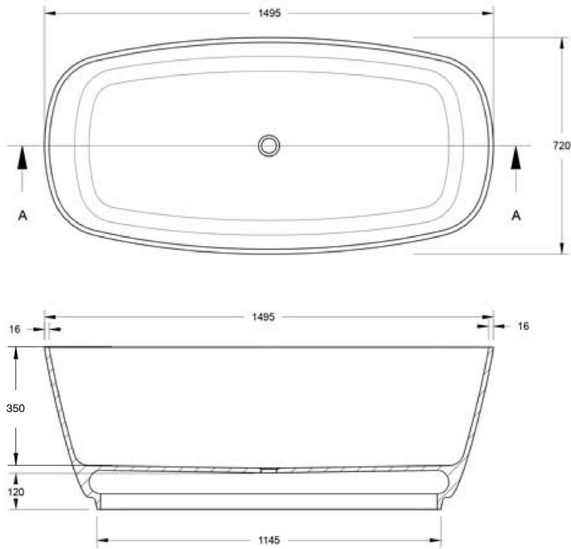
MALDON 150 X 72 TITANCAST BATH
