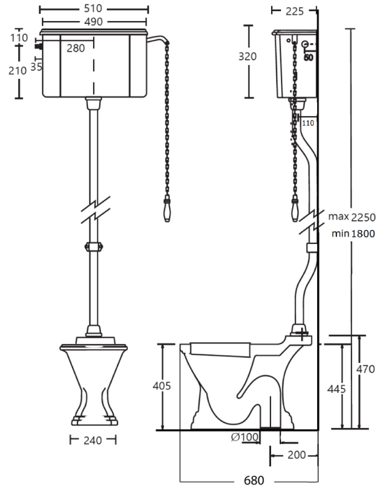
BIRMINGHAM TOILET S TRAP WITH HIGH LEVEL CISTERN
