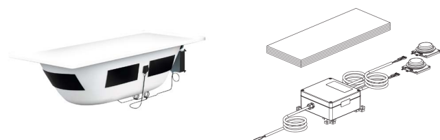
SOUND WAVE
